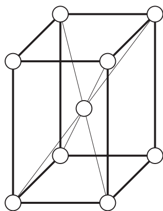
Body-centered lattice
