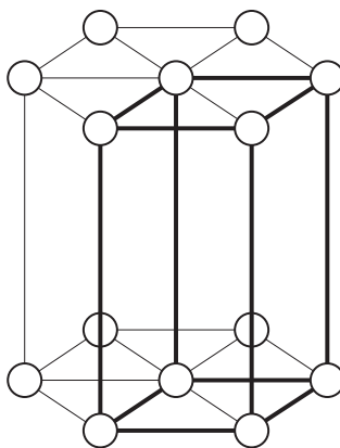
Hexagonal lattice
