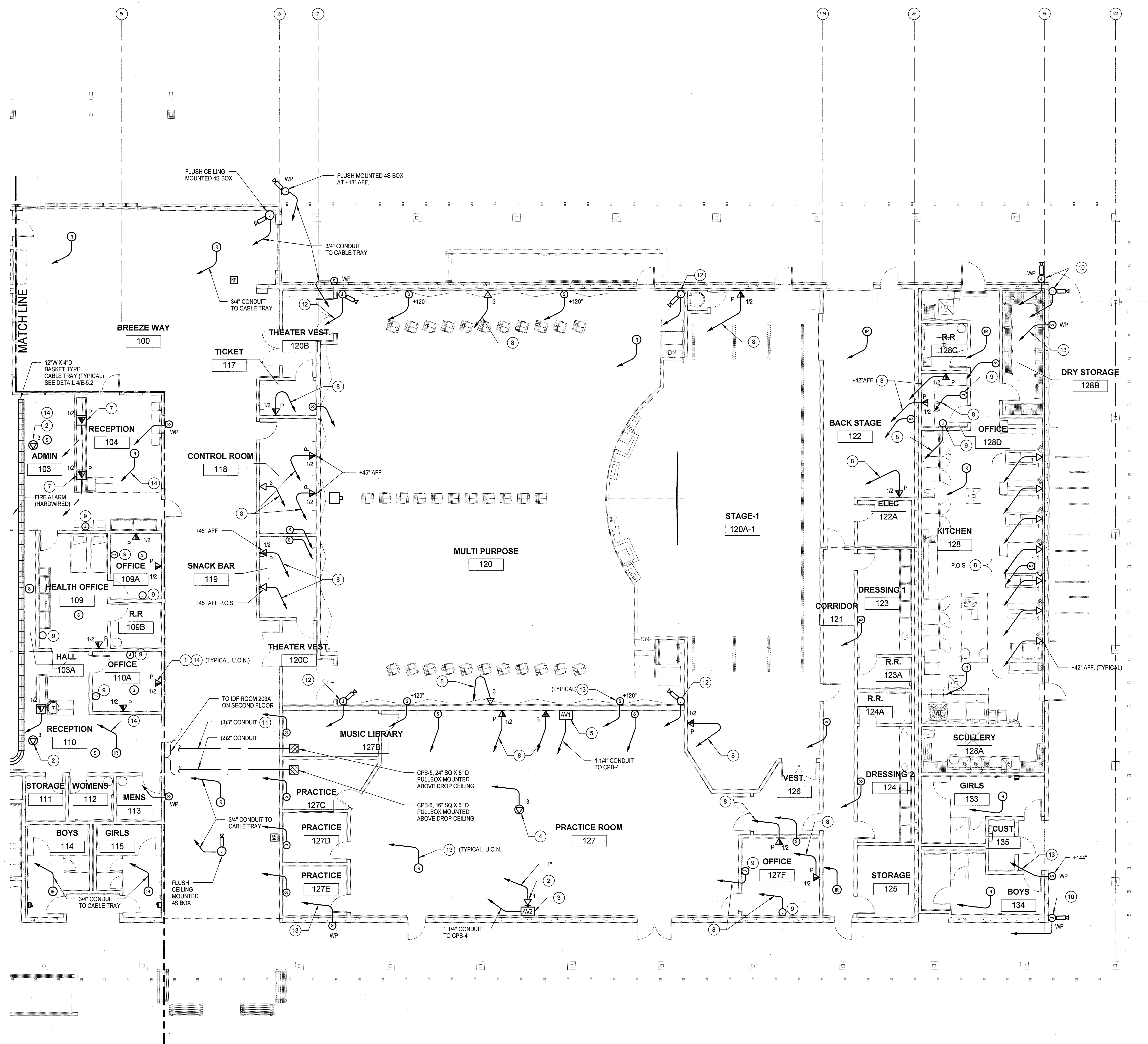
1 LEVEL 1 SIGNAL PLAN - EAST SCALE: 1/8" = 1'-0"
